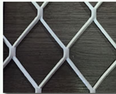
Chapa expandida espessura 1/8" (3,00mm) malha 50x100mm
