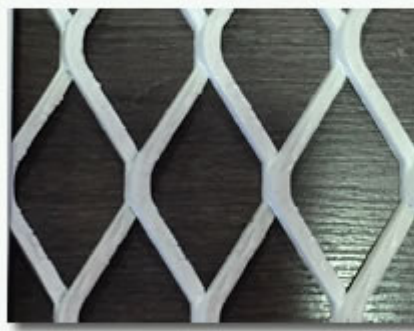
Chapa expandida espessura 3/16" (4,75mm) malha 38x75mm
